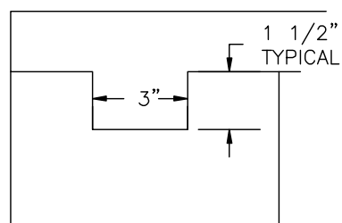
8" WALL-KEY DETAIL
