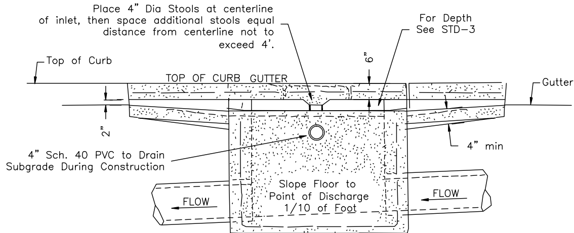
ELEVATION (Double-Wing Shown)
