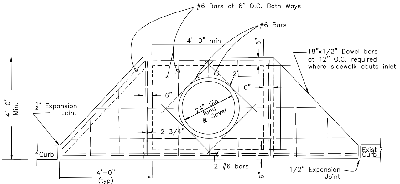
PLAN (Double-Wing Shown)
