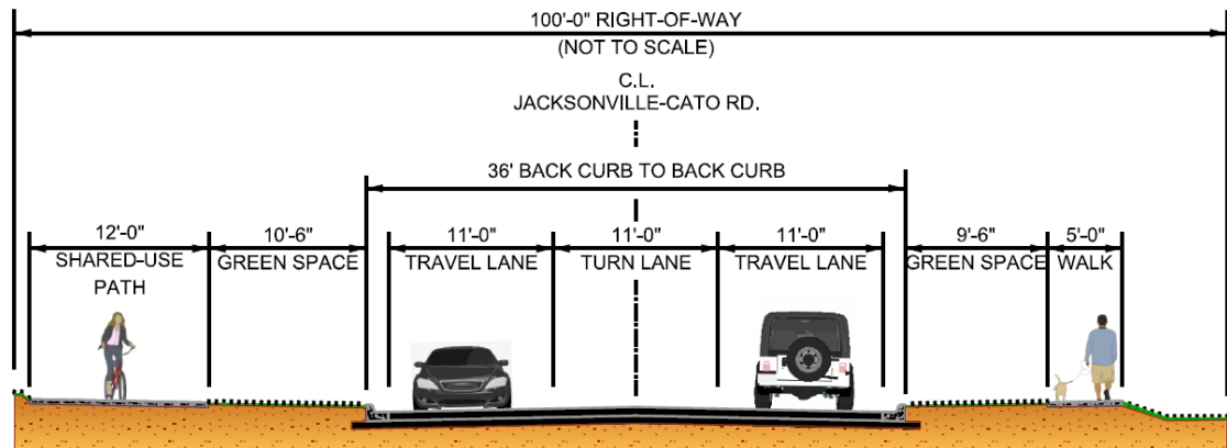
TYPICAL SECTION PROPOSED DESIGN PHASE 1
