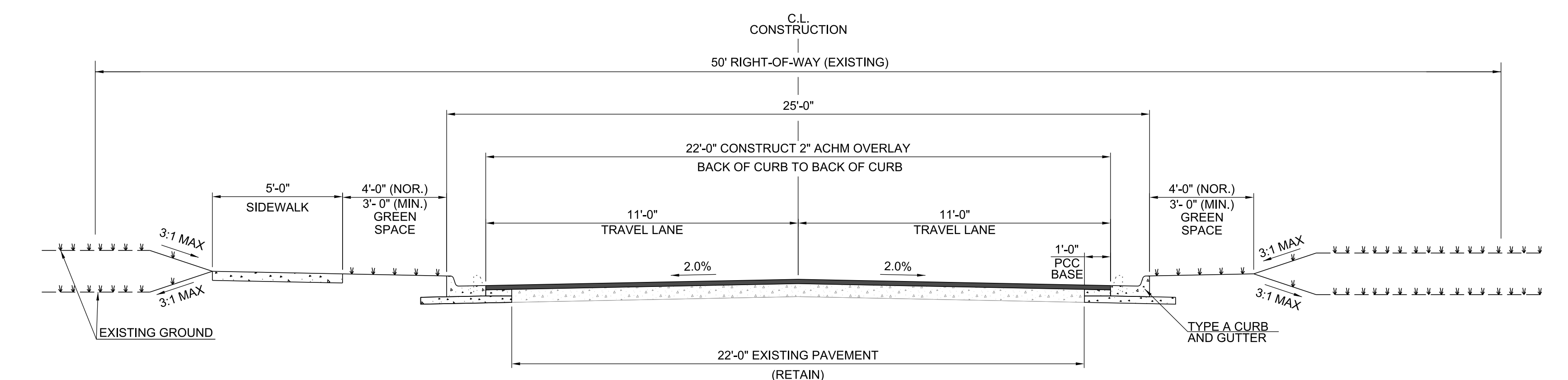
(RE TA IN) TYPICAL SECTION (SIDEWALK ON ONE SIDE) COUNTRY CLUB RD.
