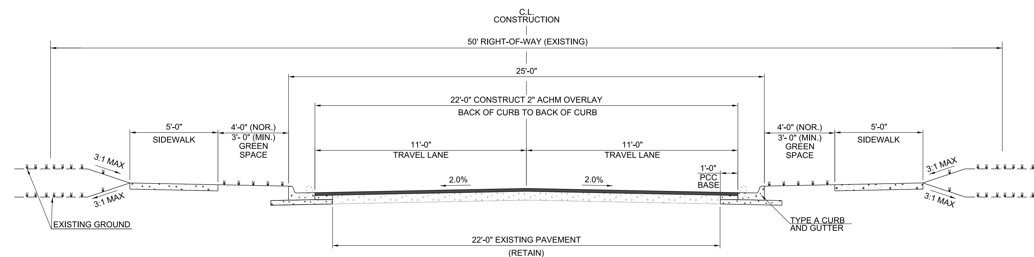
(RE TAIN) TYPICAL SECTION (SIDEWALK ON BOTH SIDES) COUNTRY CLUB RD.
